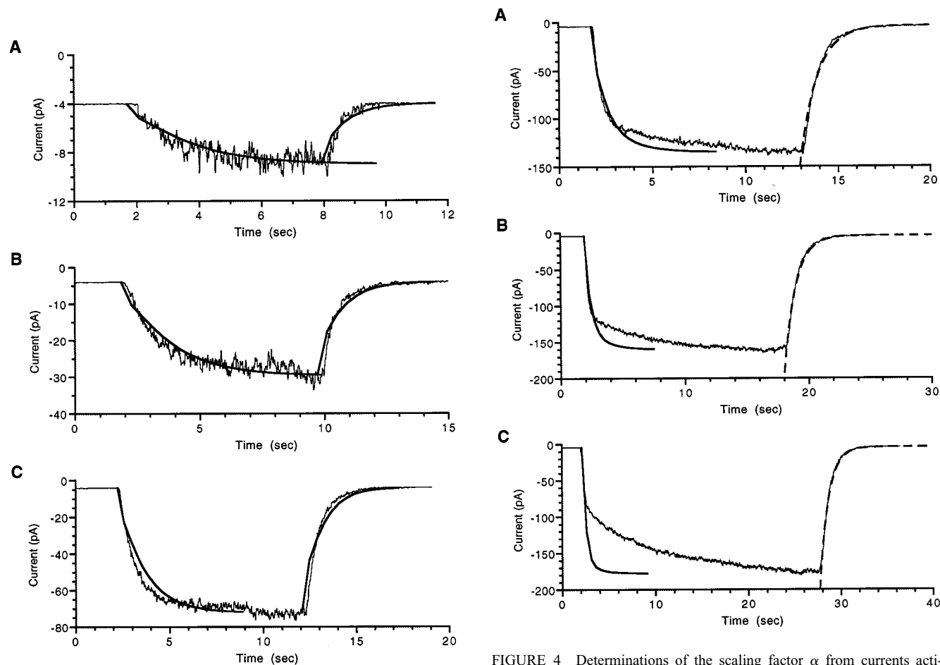
FIGURE 3 Determinations of the scaling factor \alpha from currents activated by low concentrations of cAMP. ( A ) Scaled fits of the template J(T) (thick lines) to the current record (thin line) for the 0.5 \mu\text{M} cAMP step in Fig. 1. The scaling factor \alpha was 0.25 \text{s}^{-1} and 0.30 \text{s}^{-1} for the rising and the falling phase, respectively. ( B ) Template fits for the 1 \mu\text{M} cAMP step in Fig. 1. \alpha = 0.25 \text{ s}^{-1} for both the rising and falling phases. ( C ) Template fits for the 2 \mu\text{M} cAMP step in Fig. 1. \alpha = 0.30 \text{ s}^{-1} for the rising phase and 0.25 \text{s}^{-1} for the falling phase.
