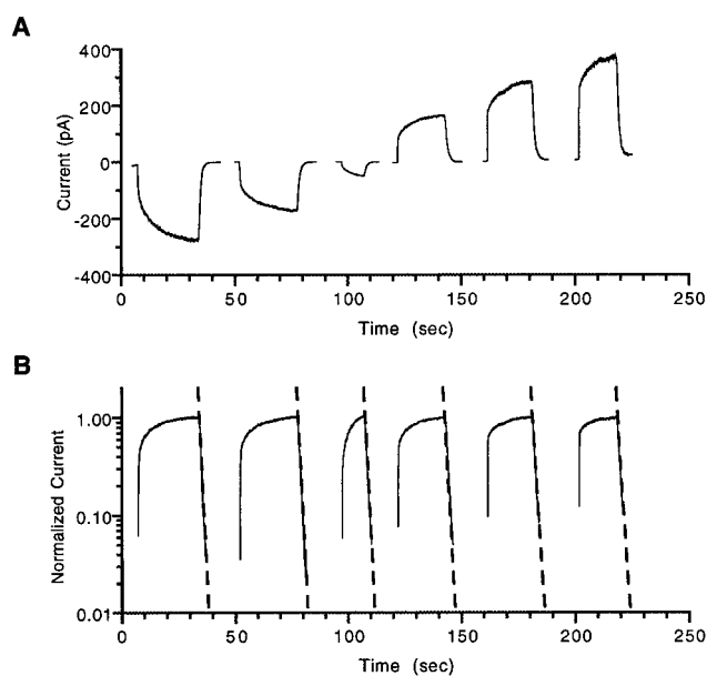
FIGURE 5 Dependence of the amplitude and kinetics of the cAMP-activated current on membrane voltage. ( A ) Currents elicited by 20 \text{ }\mu\text{M} cAMP at different voltages. Leak currents have been subtracted. From left to right, membrane voltage was held at -60 , -40 , -20 , +20 , +40 , and +60 mV. ( B ) Normalized currents from ( A ) plotted on a logarithmic scale. The time scale is the same as in ( A ). The dashed lines are exponential fits to the falling phases. The decay rates were (from left to right) 1.30 , 1.04 , 1.10 , 0.95 , 1.11 , and 1.14 \text{ s}^{-1} . Same cilium as in Fig. 1.
